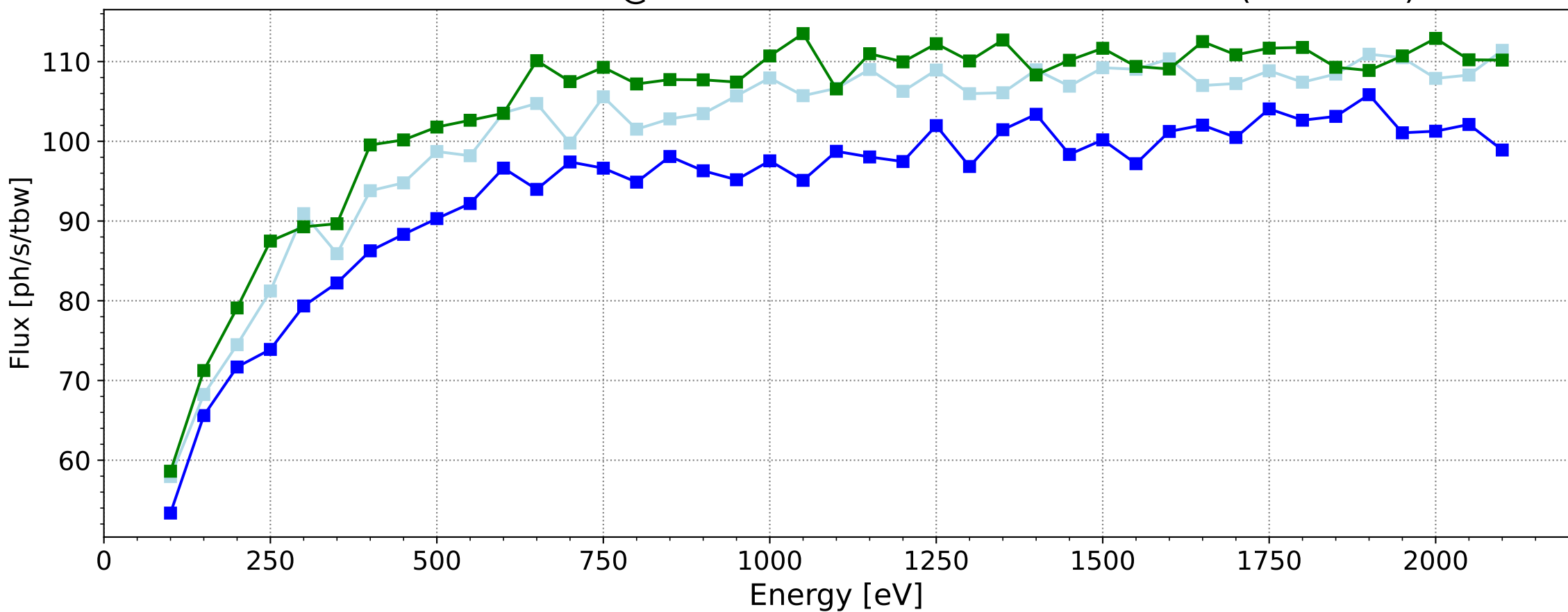
BESSY II vs. BESSY III @ 56 m standard PGM-BL PerMil flux (errors off)
